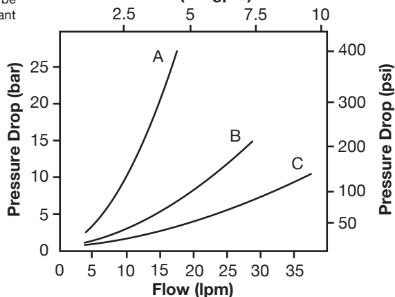
Typical Pressure Drop Curve #
